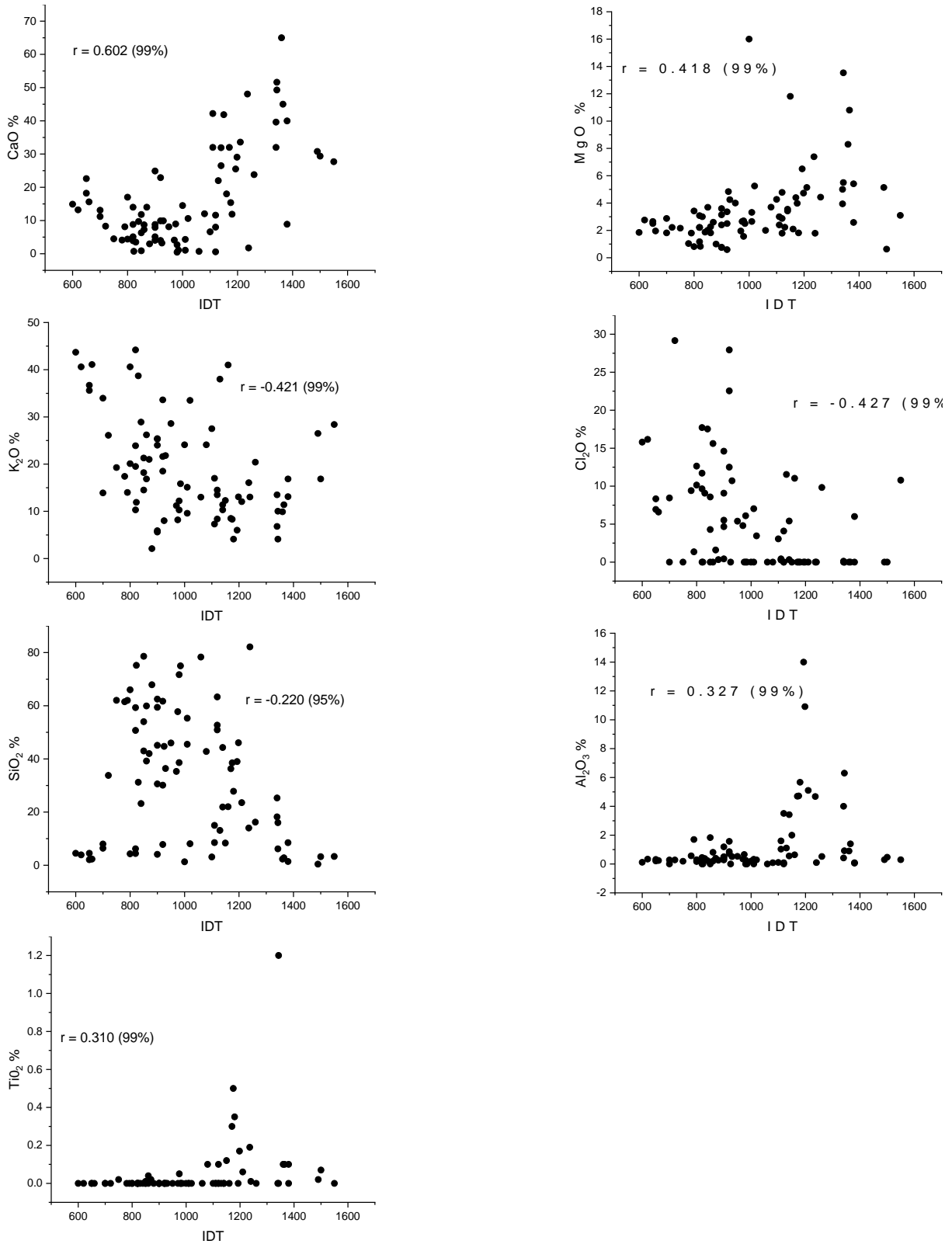
Fig. S2. Some significant correlations of ash chemical compositions against IDT (80 samples).
