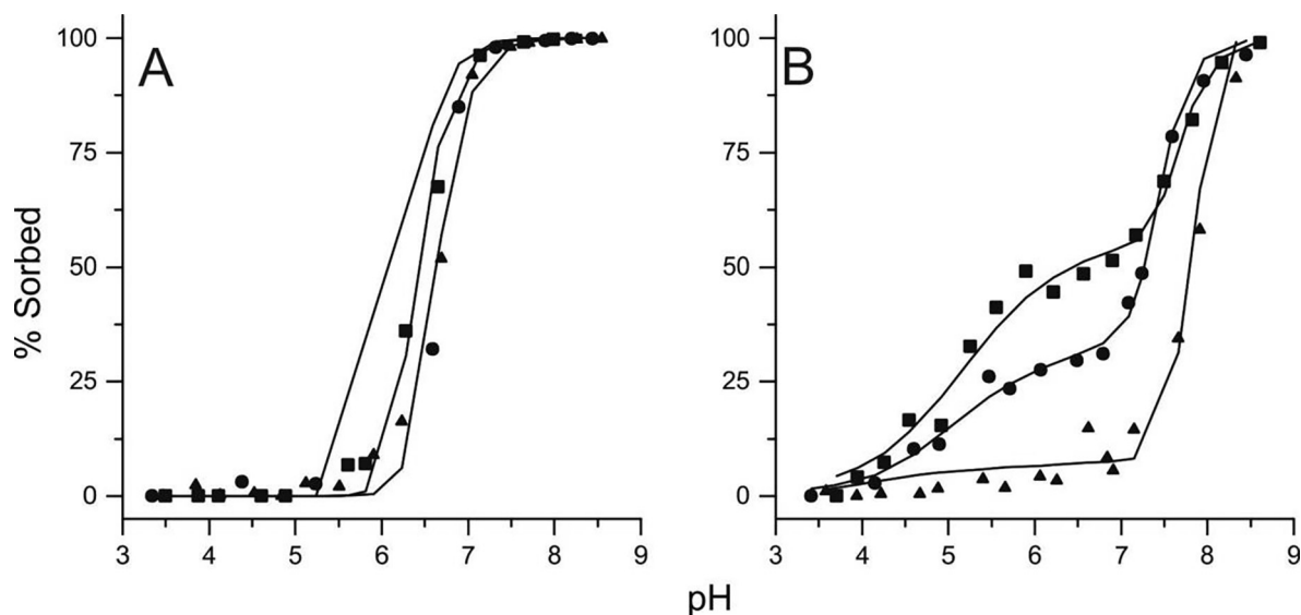
Fig. 2. Co sorption (at 10^{-4} mol L -1 Co total concentration, equating to 0.58 wt% Co sorbed at 100% sorption for Fh and 0.058 wt% Co sorbed at 100% sorption for Ka) to Fh (A) and Ka (B) as a function of pH; conducted at room temperature at a range of ionic strengths ( 10^{-3} , squares; 10^{-2} , circles; and 10^{-1} , triangles, mol L -1 NaNO 3 ). Solid lines are the surface complexation model fits for each system.
