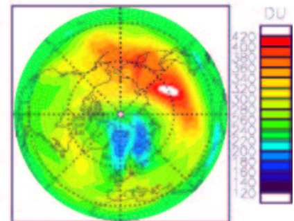
SLIMCAT TOZ on 6/12/2002
