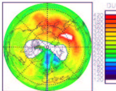
GOME TOZ on 6/12/2002
