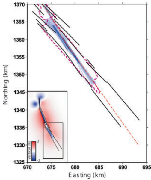
Figure 4. Density plot of the set of best fitting dykes for the seven post 2005 intrusions, black lines show the location of normal faults traced from DEM. Dashed purple line is the outline of the area of subsidence associated with the 2005 September intrusion (Wright et al. 2006; Rowland et al. 2007). The dashed red line is the chosen simplified geometry for the distributed opening model described in Section 2.3.2. The subplot shows the modelled vertical displacements from the 2005 September intrusion. Coordinates are in UTM Zone 37.
